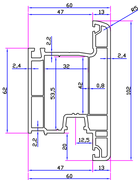
60 OUTWARD OPENİNG DOOR SASH
