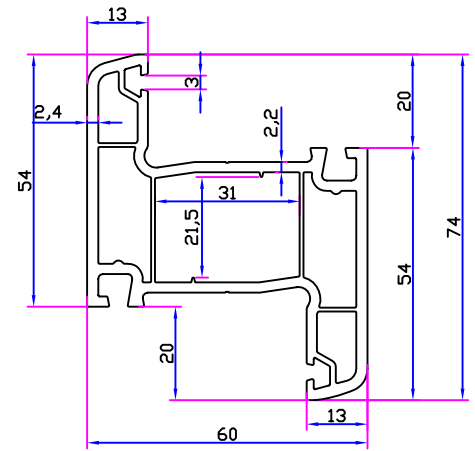
60 OUTWARD MULLION SERİE
