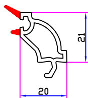
DOUBLE GLAZING BEAD
