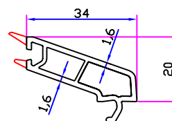
5-6mm SINGLE GLAZING BEAD
